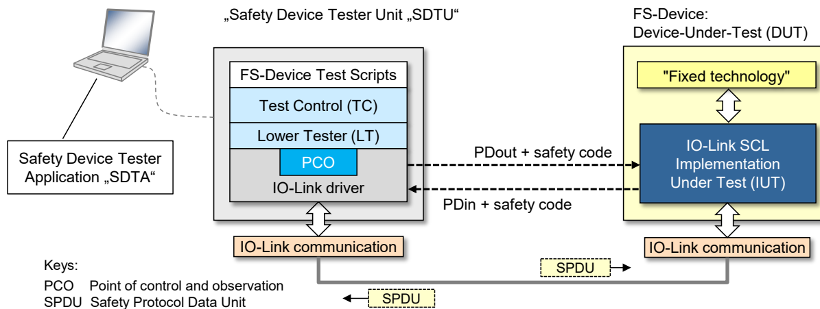
Figure A.11 – Principle of FS-Device SCL testing
