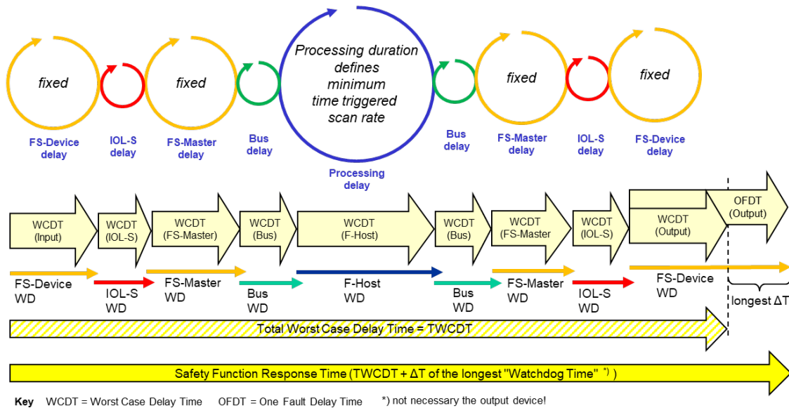
5658 Figure 16 – SFRT including IOL-S and FSCP
