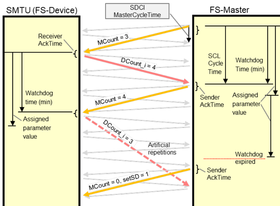
5663 Figure 17 – Test of the FS-Master watchdog
