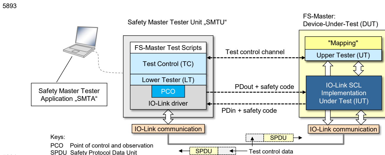
5894 5895 Figure A.7 – Principle of FS-Master SCL testing
