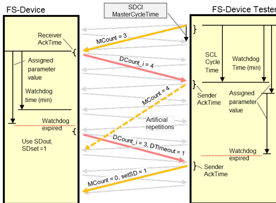
Figure 11 – Principle of FS-Device watchdog timer test
