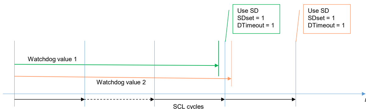
Figure 12 – Influence of SCL sampling effects
