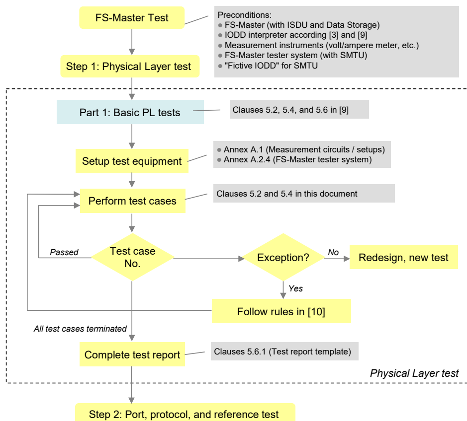
Figure 7 – Step 1 of the FS-Master test sequence (PL)
